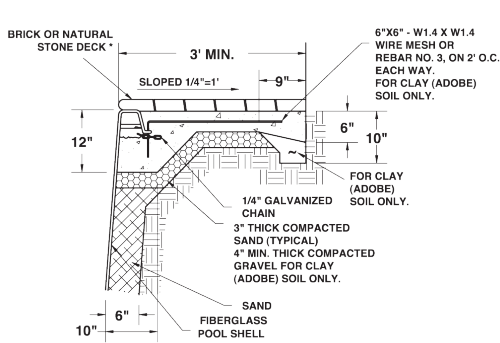
Figure 6 Concrete Deck with Brick or Stone
