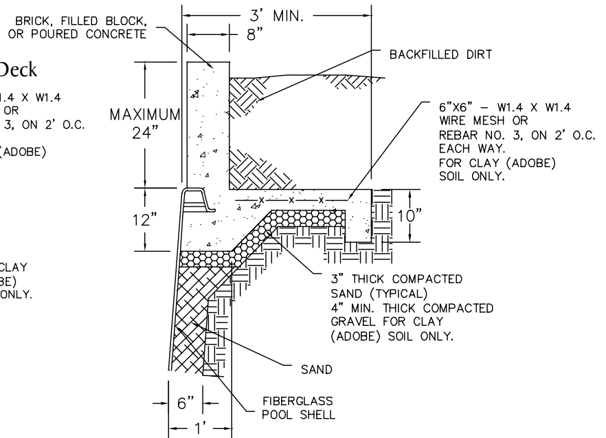
Figure 9 Typical Bond Beam Construction
