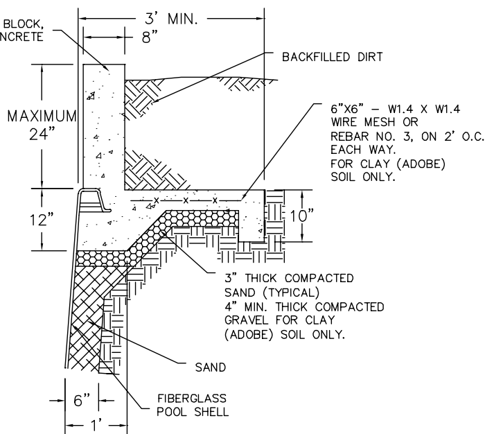
Figure 9 Typical Bond Beam Construction
