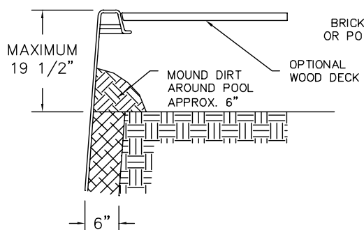
Figure 8 Typical above Ground Installation
